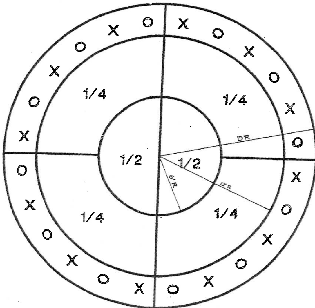
PRIMARY STRIPING PLAN - ITEM 1 1/4" = 1'-0"
